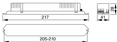
Driver
