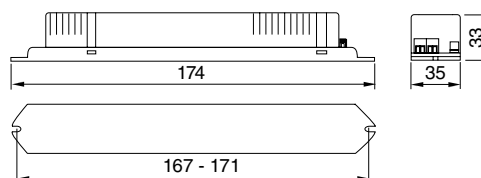
Driver
