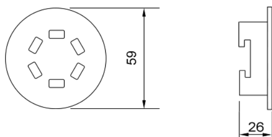
Dimensiones driver (mm)
